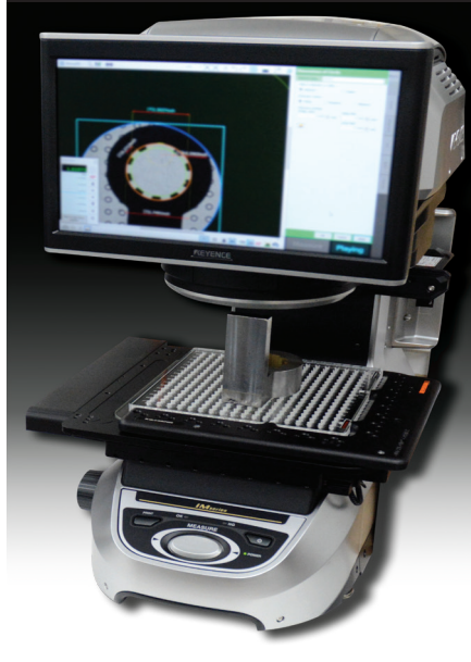
Visual Inspection System
